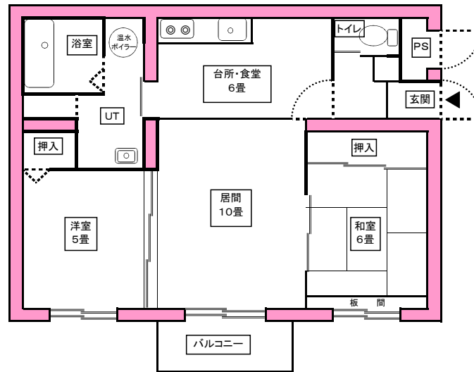
2DK-B (67.26㎡)
